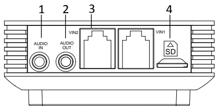
Figure 1-6 The Type C Front Panel
