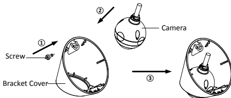
Figure 2-35 Place the Camera in Bracket Cover
